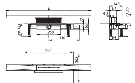
Shower channel kit CeraWall Pure Plan, DN 40
