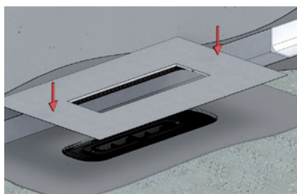
2. Fasten the sealing sleeve with a click on the drain body, then seal off against water
