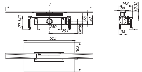
Shower channel kit CeraFloor Pure, DN 50
