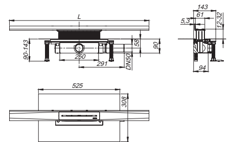
Shower channel kit CeraWall Pure, DN 50
