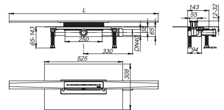
Shower channel kit CeraFloor Pure Plan, DN 40
