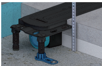
1. Insert the drain body into the screed
