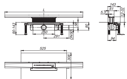
Set douchegoot CeraWall Pure, DN 50
