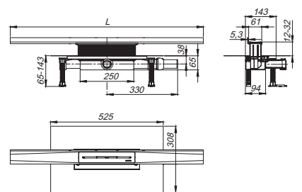
Set douchegoot CeraWall Pure Plan, DN 40
